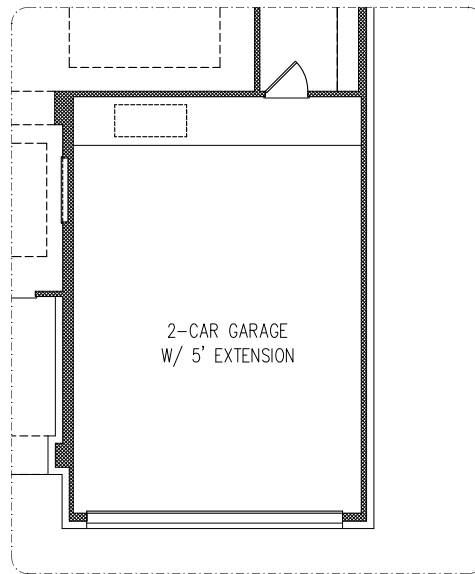
OPTIONAL GARAGE W/ 5' EXT.
