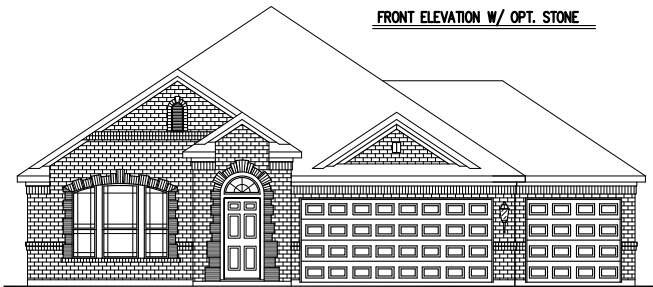
FRONT ELEVATION W/ OPT. 3 CAR
